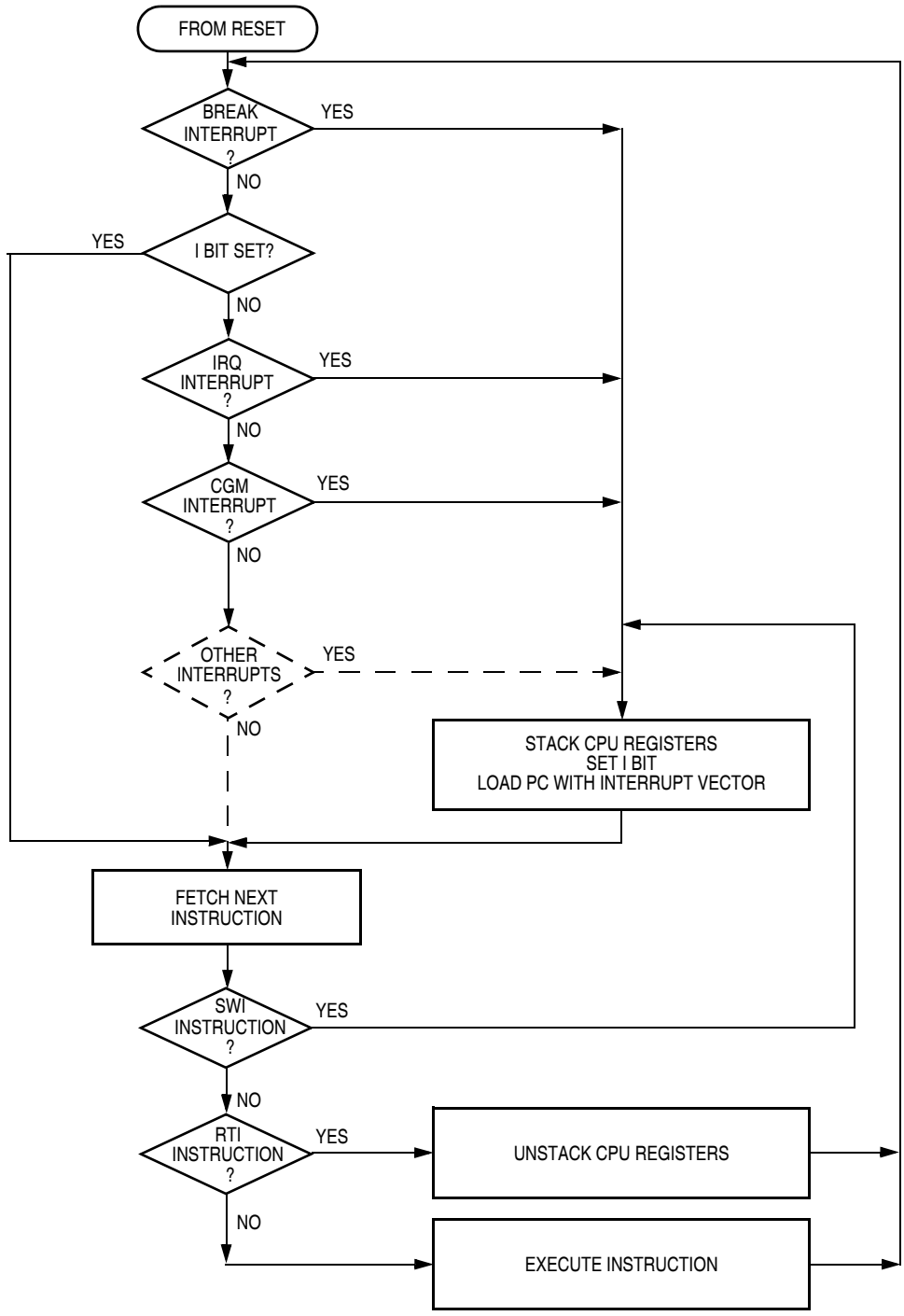
Figure 14-10. Interrupt Processing
